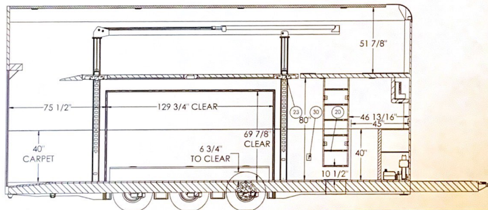
INTERIOR ROADSIDE SECTION B-B
