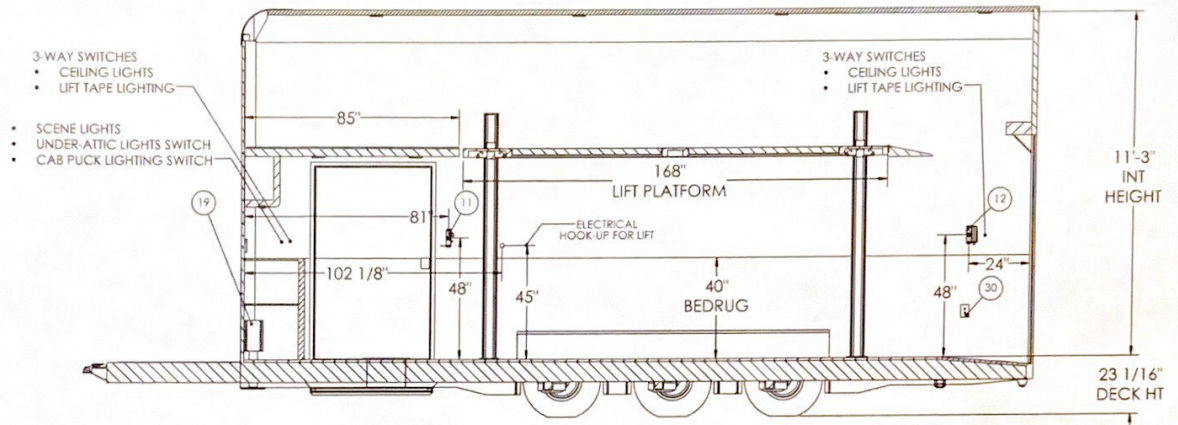
INTERIOR CURBSIDE SECTION A-A
