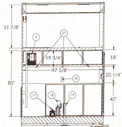
INTERIOR FRONT SECTION C-C
